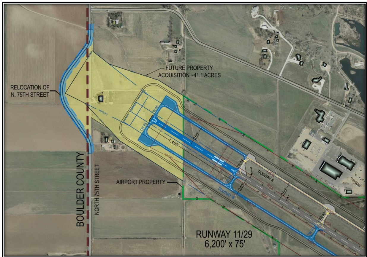
FIGURE 5-7 - ALTERNATIVE 5 - 1,400' EXTENSION
