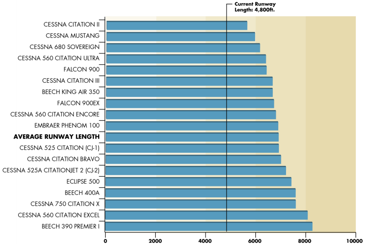
GRAPH 4-2 – PART 135 CHARTER AIRCRAFT LANDING DISTANCE REQUIRED AT LMO (DRY CONDITIONS)
