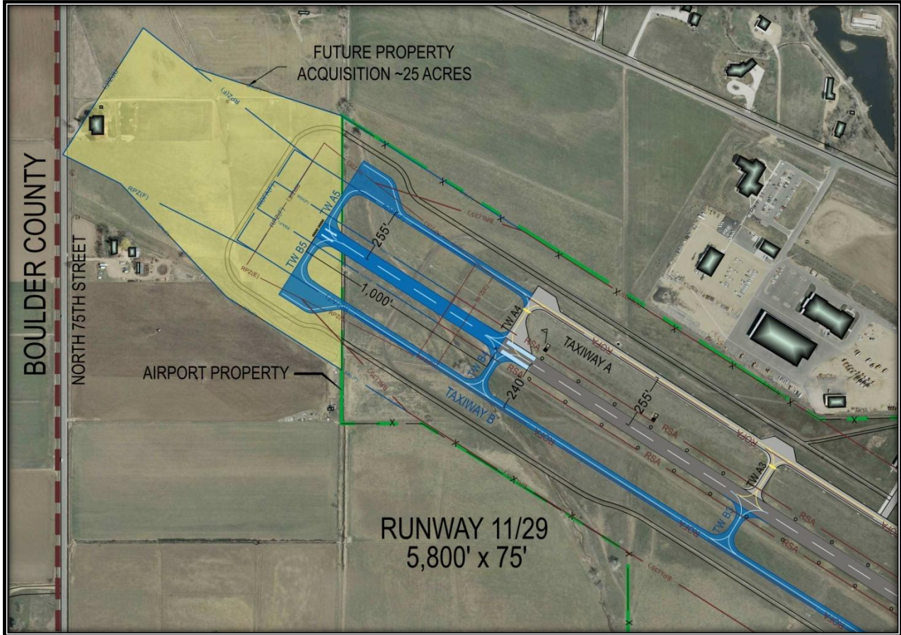
FIGURE 5-5 - ALTERNATIVE 3 - 1,000' EXTENSION
