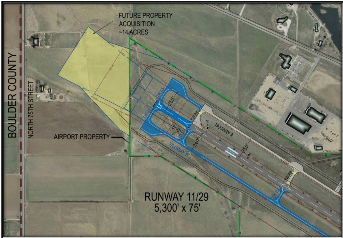
FIGURE 5-4 - ALTERNATIVE 2 - 500' EXTENSION
