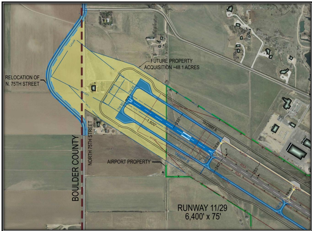
FIGURE 5-8 - ALTERNATIVE 6 - 1,600' EXTENSION
